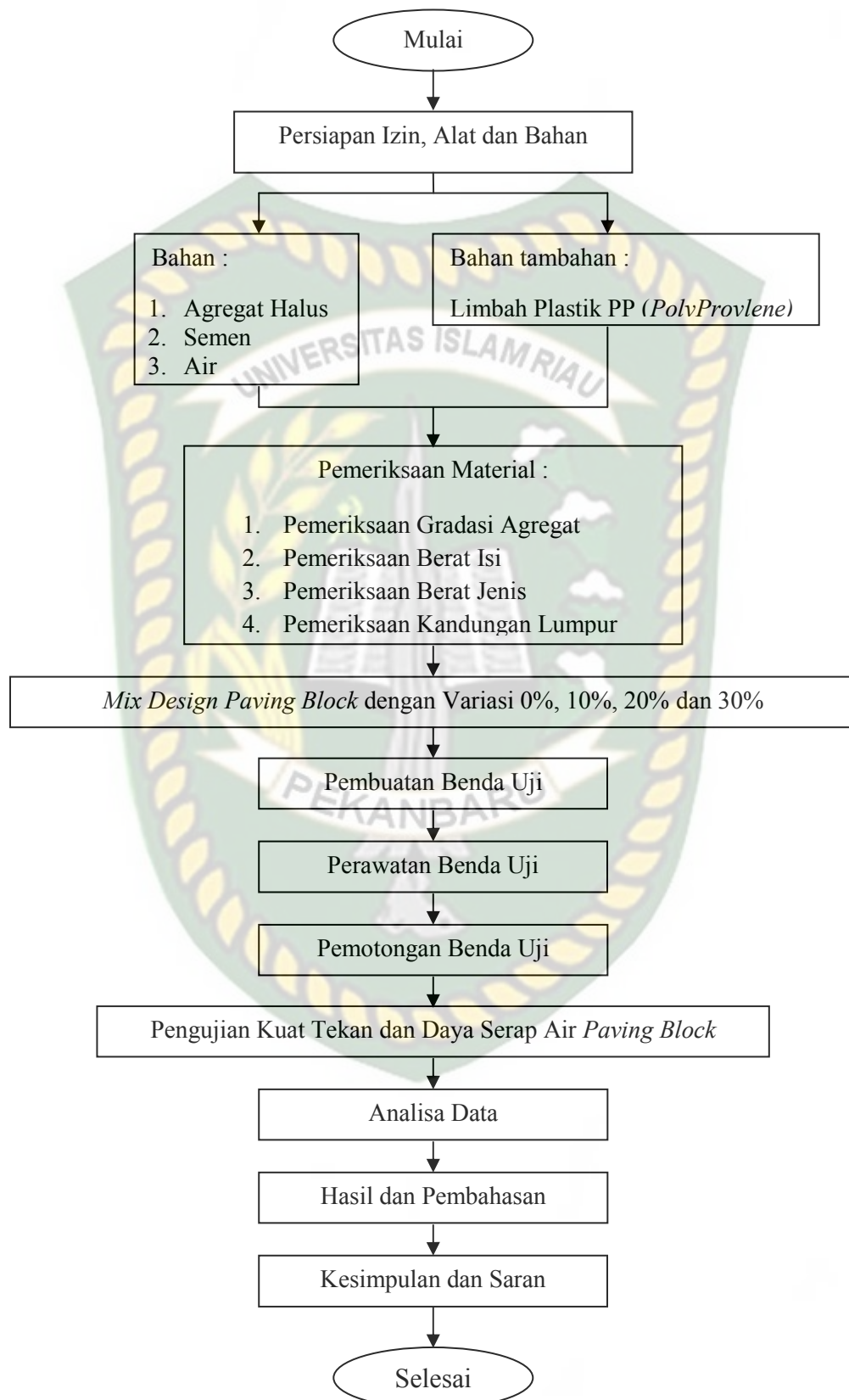
Gambar 4.22 Diagram Alir Penelitian
