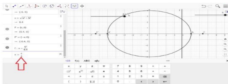
Figure 1. Geogebra display results for Ellipse material
