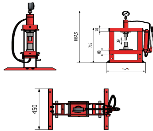
Figure 7. Side, front and top view
