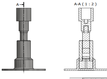
Figure 6. Construction of mold press
