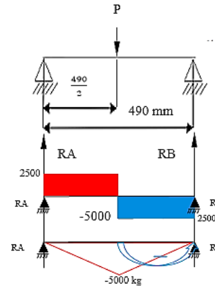
Figure 10. Maximum moment
