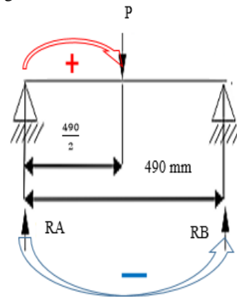
Figure 8. Vertical support reaction A
