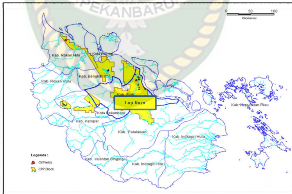
Gambar 3.1. Peta Lokasi Reservoir Lapangan Raya (BOB PT. BSP)
