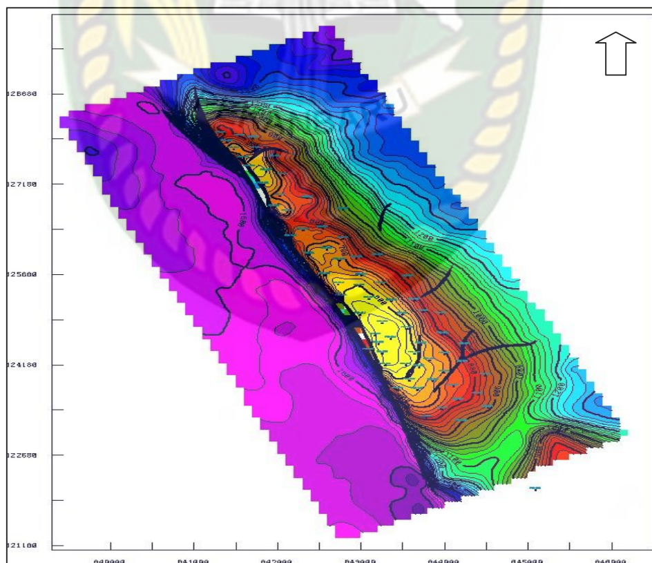
Gambar 3.5. Struktur Reservoir Lapangan Raya (BOB PT.BSP)
