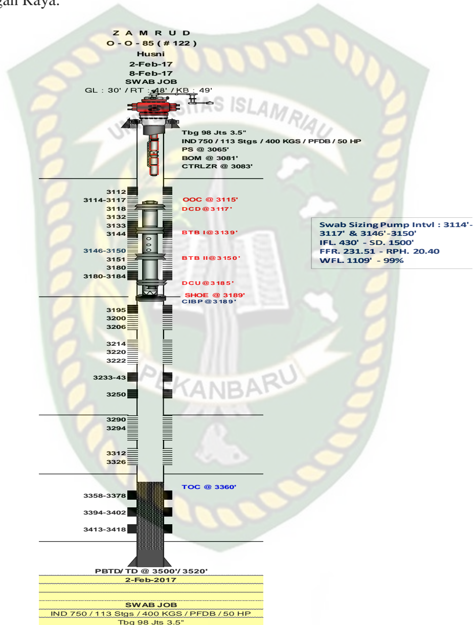
Gambar 3.6. Well schematic R122 (BOB PT. BSP Well)
