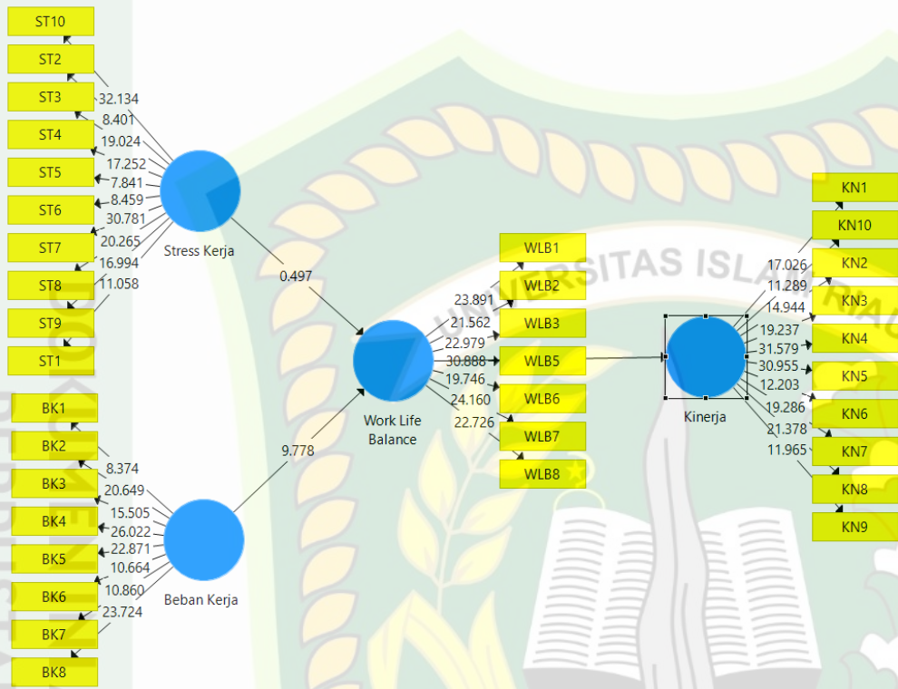
Figure 2. Bootstrapping
