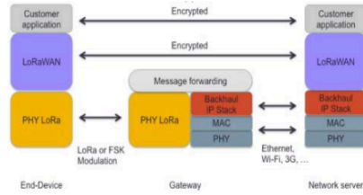
Fig. 6. LoRaWAN (a) system and (b) protocol architecture
