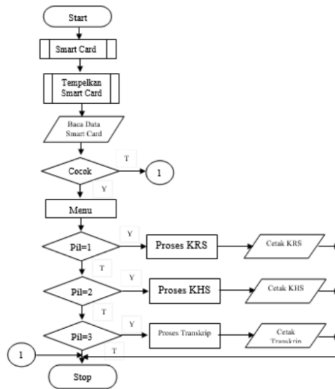
Gambar 4. Flowchart Smart Card
