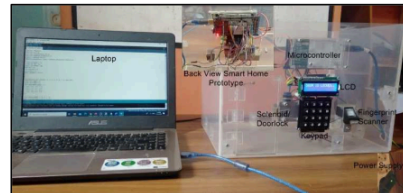
Fig. 3. Hardware prototype design
