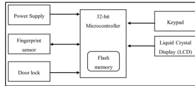
Fig. 2. The proposed hardware design of the FAS
