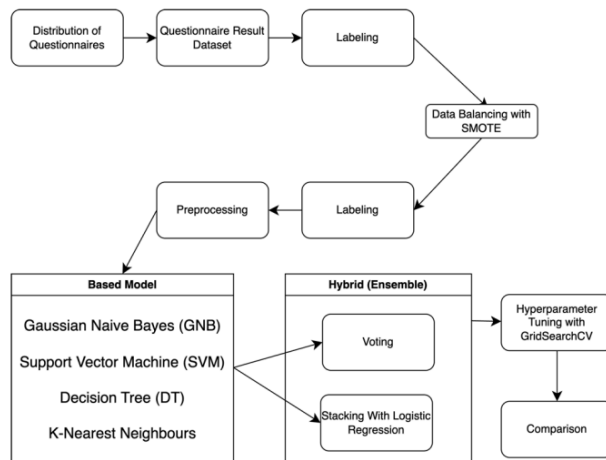
Figure 1. Research Methodology
