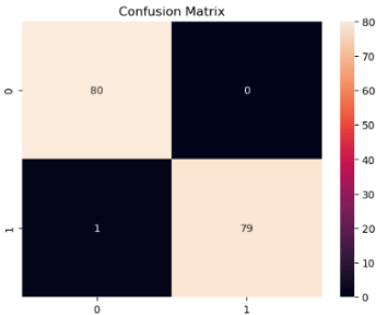
Figure 3. Confusion Matrix
