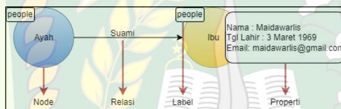
Gambar 2. 3 Contoh Basis Data Graf
