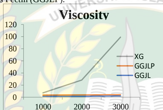
Fig. 4. Viscosity Test Results Of Xanthan Gum (XG), Green Grass Jelly Leaves (GGJL), Green Grass Jelly Leaves Pectin (GGJLP).
