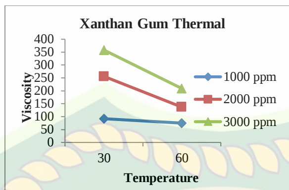
Fig. 10. Xanthan Gum Thermal Test Chart.
