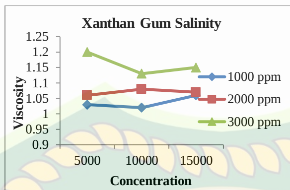
Fig. 5. Xanthan Gum Salinity Test Graph.
