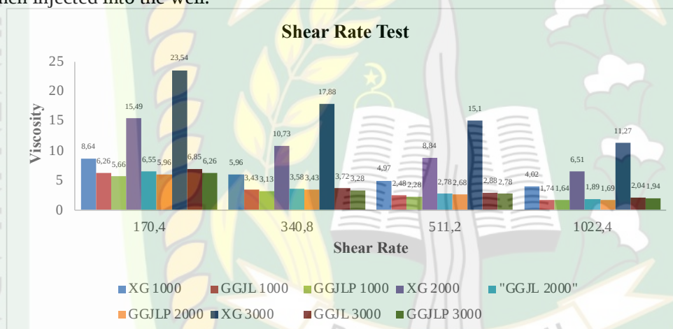
Fig. 8. Graph Of Testing Shear Rate 1000, 2000, And 3000 Ppm On Xanthan Gum (XG), Green Grass Jelly Leaves (GGJL), And Green Grass Jelly Leaves Pectin (GGJLP).
