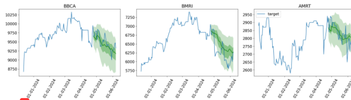
Figure 10: Optimal Parameters for Multi Time Series: BBKA, AMRT, and BMRI Stocks with TFT
