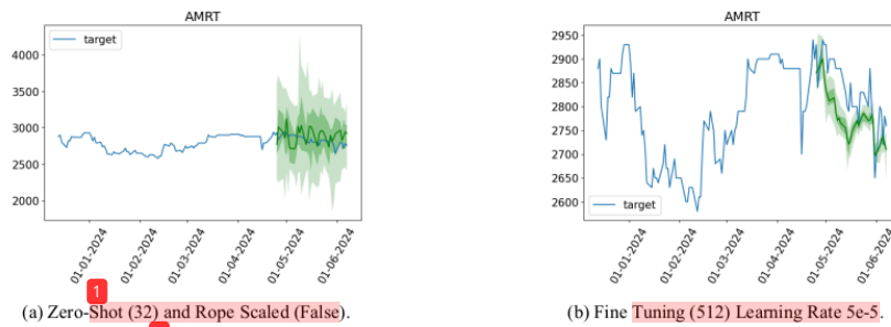
Figure 6: Optimal Parameters for Univariate Time Series (Lag-Llama - AMRT Stock).
