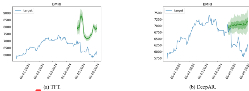
Figure 5: Optimal Parameters for Univariate Time Series (Baseline Models - BMRI Stock).
