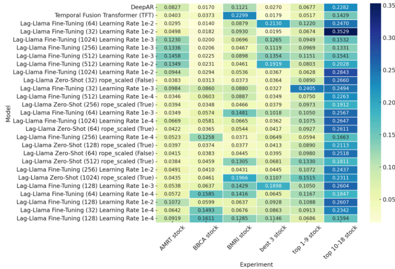
Figure 1: CRPS Scores of All Models Across Six Experimental Settings. Lighter yellow cells indicate lower CRPS values and thus better probabilistic forecasting performance, while darker blue cells represent higher CRPS values and weaker performance.
