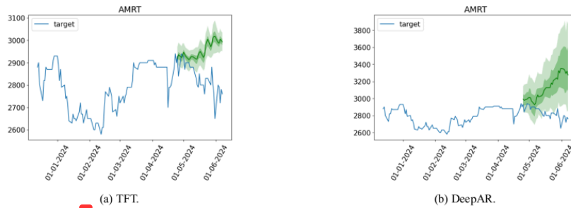
Figure 7: Optimal Parameters for Univariate Time Series (Baseline Models - AMRT Stock).
