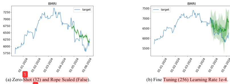
Figure 4: Optimal Parameters for Univariate Time Series (Lag-Llama - BMRI Stock).
