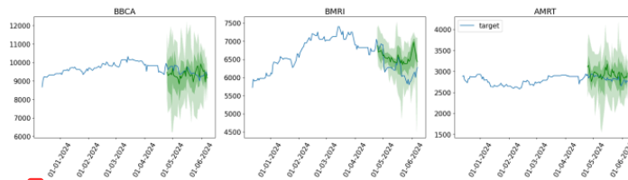
Figure 8: Optimal Parameters for Multi Time Series: BBKA, AMRT, and BMRI Stocks with Zero-Shot (32) and Rope Scaled (False)
