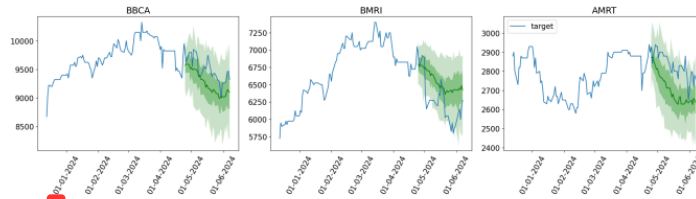
Figure 11: Optimal Parameters for Multi Time Series: BBKA, AMRT, and BMRI Stocks with DeepAR
