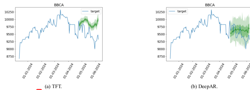
Figure 3: Optimal Parameters for Univariate Time Series (Baseline Models - BBKA Stock).
