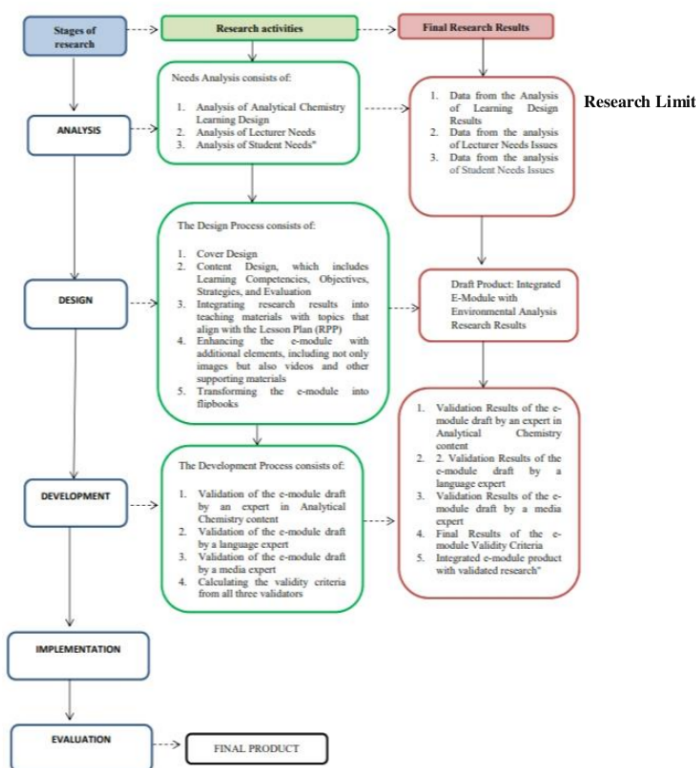
Figure 1. Research Flowchart
