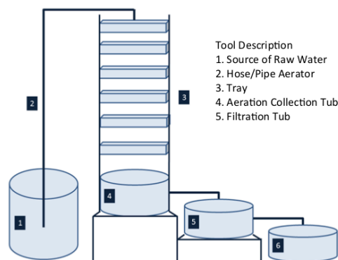
Figure 1. Aeration-Filtration Tool Scheme
