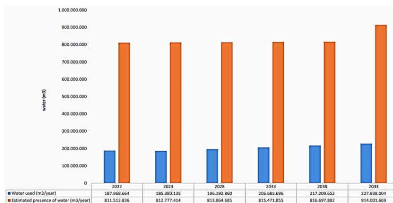
Figure 6 | Water balance (m³/year) in the Kampar regency in the Kampar watershed.
