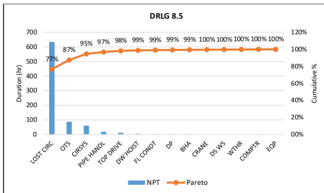
Fig. 4. Pareto Chart DRLG 8-1/2*
