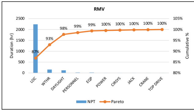
Fig. 3. Pareto Chart RMV
