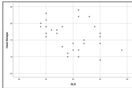
Gambar 1. Scatter Plot
