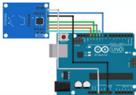
Figure 5: An Arduino module with RFID reader.
