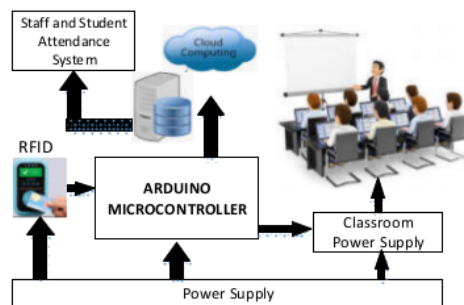
Figure 1: Block diagram of student attendance system.
