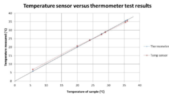
Fig. 7. Temperature sensor results vs thermometer
