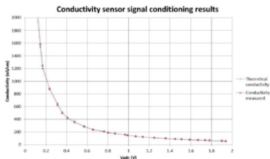
Fig. 8. Electrical conductivity test results for sensor node
