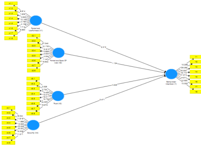
Gambar 2. Diagram Path PLS Algoritma
