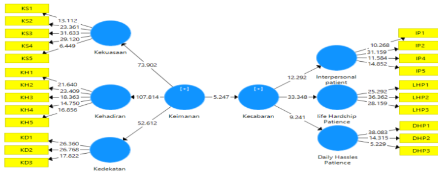
Gambar 2. Analisis Inner Weight
