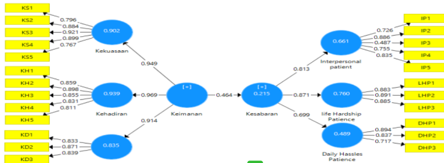
Gambar 1. Analisis Outer Model
