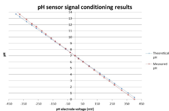
Figure 7: Water pH sensor test between theoretical and actual measurements.
