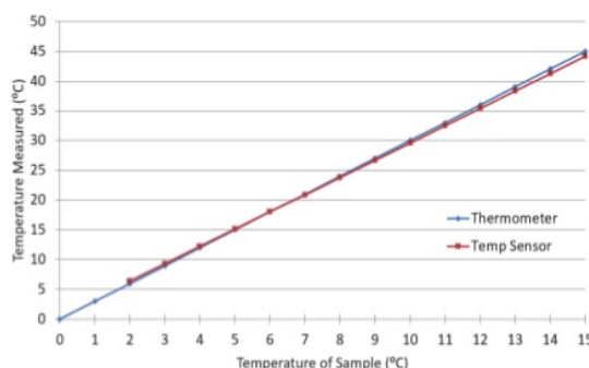
Fig. 5. Comparison of temperature obtained from the proposed system to that obtained using conventional method using thermometer.
