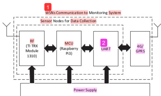
Fig. 2. Proposed diagram for WSNs sink node communication to sensors.
