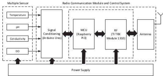
Fig. 1. Block diagram of multiple sensors system.
