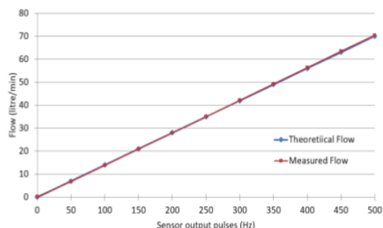
Fig. 8. Water flow meter test versus theoretical analysis.
