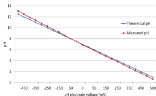
Fig. 7. Water pH test results versus theoretical values.
