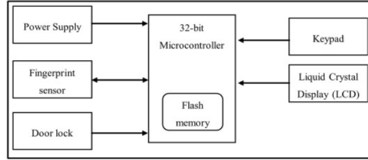
Fig. 2. The proposed hardware design of the FAS
