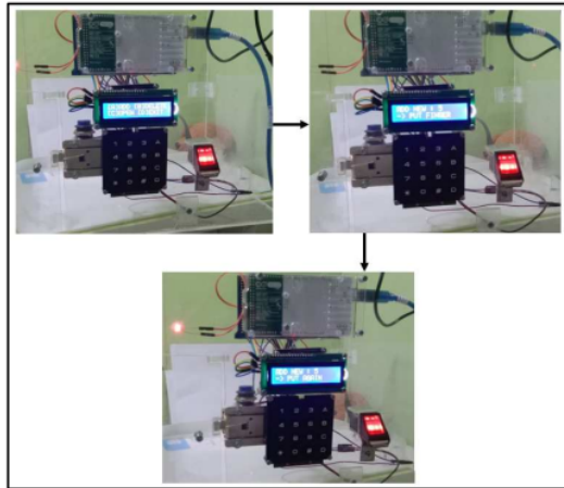
Fig. 5. Enrolment process in prototype smart home
