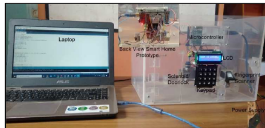
Fig. 3. Hardware prototype design
