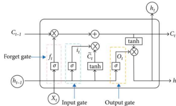
Figure 3. Structure of the RNN-LSTM algorithm.
