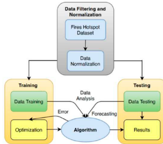
Figure 4. Block diagram analysis in data forecasting.
