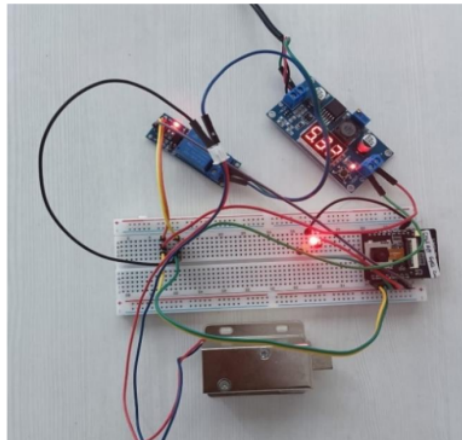
Figure 3. Hardware prototype design results
