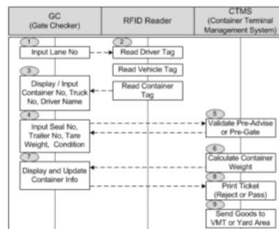
Fig. 3. Proposed business process used RFID technology.
