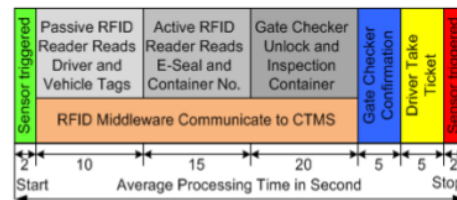
Fig. 8. Reading timeline of container in receiving area.
