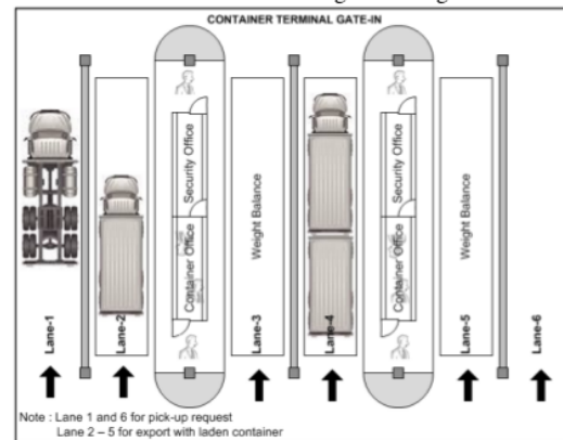
Fig. 1. Layout of container terminal gate-in.
