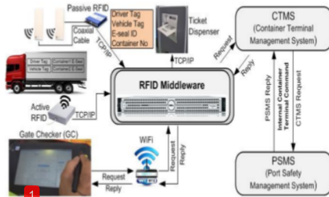
Fig. 7. Architecture of RFID system for receiving gate.
