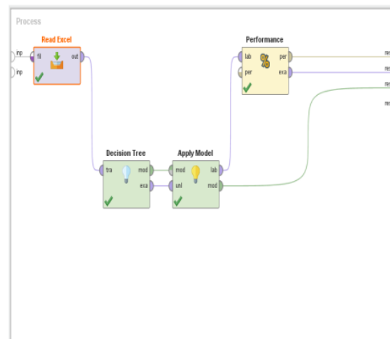
Gambar 1. Proses model penilaian 5K2S
