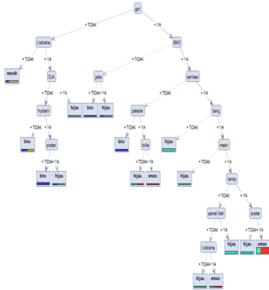
Gambar 2. Pohon keputusan (decision tree) penilaian 5K2S
