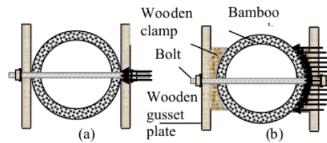
Fig. 2 Distribution of force on the bolt and wooden gusset plate to a bamboo culm (a) direct force into a bamboo culm (b) force through to a wooden clamps
