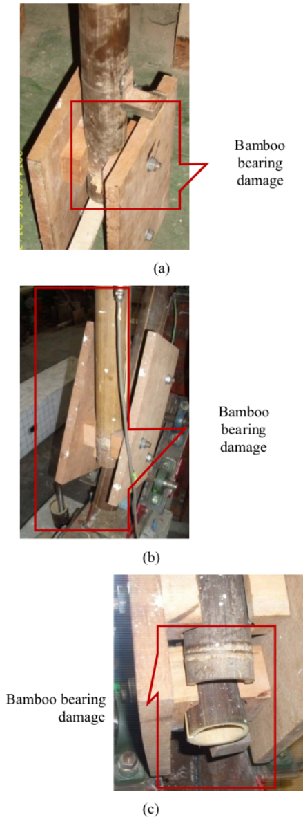
Fig. 7 Failure modes of the specimen (a) bamboo stem angle 0° (b) bamboo stem angle 30° (c) bamboo stem angle 45°
