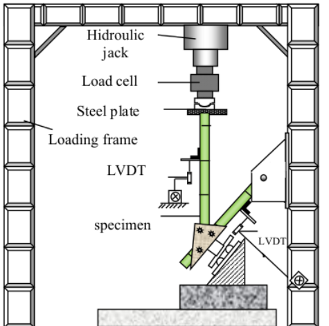
Fig. 3 Test set-up for compression tests of the specimen.
