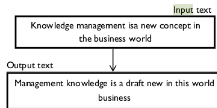
Fig 2. Stages Tokenizing
