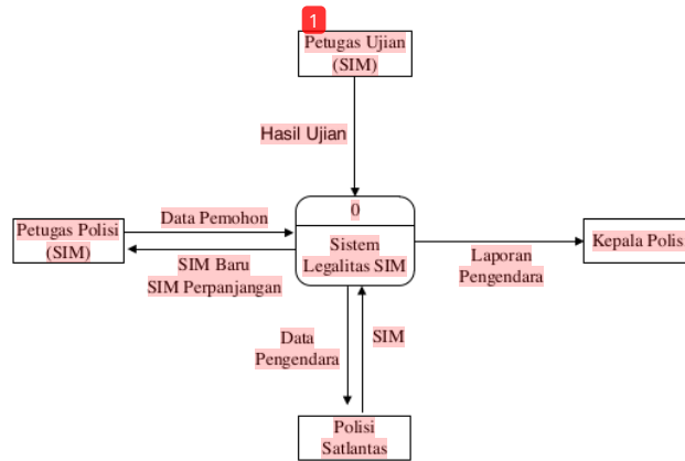
Gambar 1. Context Diagram Legalitas Surat Izin Mengemudi (SIM)
