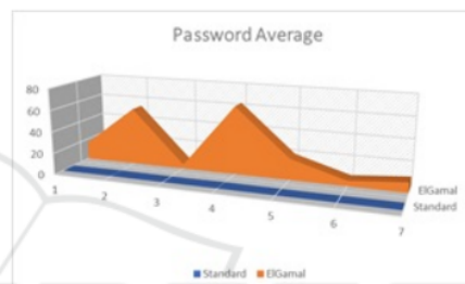
Figure 2: Password Average (Second).
