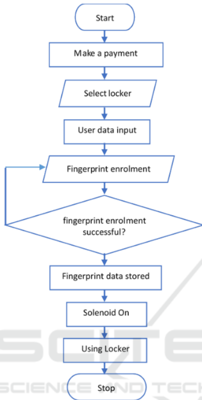
Figure 2: Flow chart locker security system
