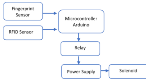
Figure 1: Hardware scheme locker security system.
