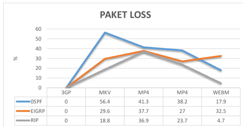
Gambar 4. Perbandingan Paket Loss Video routing OSPF, EIGRP dan RIP
