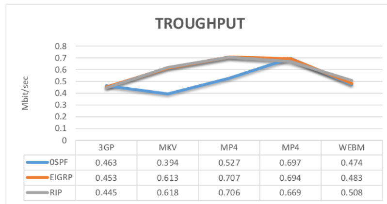
Gambar 2. Perbandingan Throughput routing OSPF , EIGRP dan RIP
