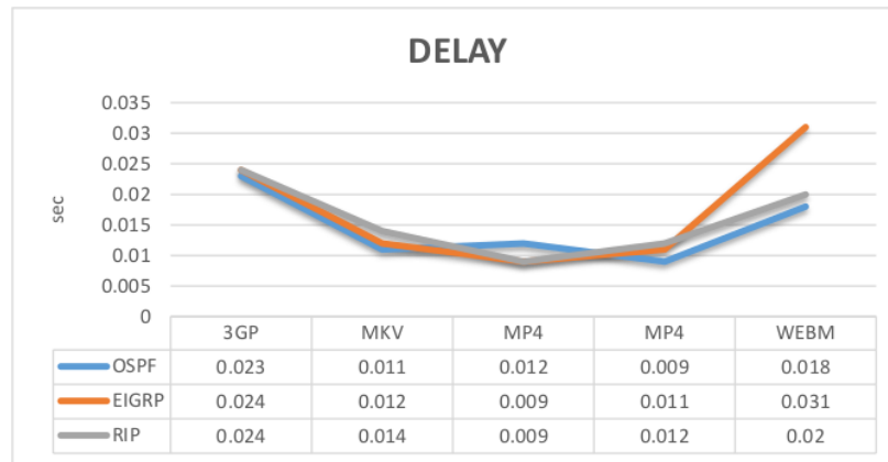
Gambar 3. Perbandingan Delay routing OSPF, EIGRP dan RIP
