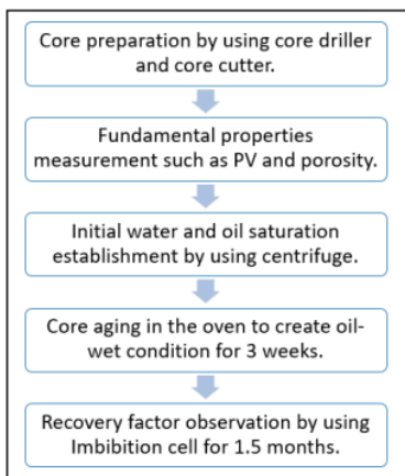
Figure 1. Workflow spontaneous imbibition test
