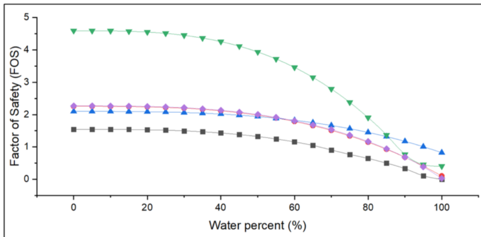
FIGURE 7. Sensitivity analysis to determine the percentage of water required to induce failure (FOS <1.00) as observed on site on several potential failures. The FOS values decrease as water percentage within the discontinuity increases, eventually falling below FOS=1. This highlights the need to consider water even in dry conditions, as Malaysia often experience torrential rains
