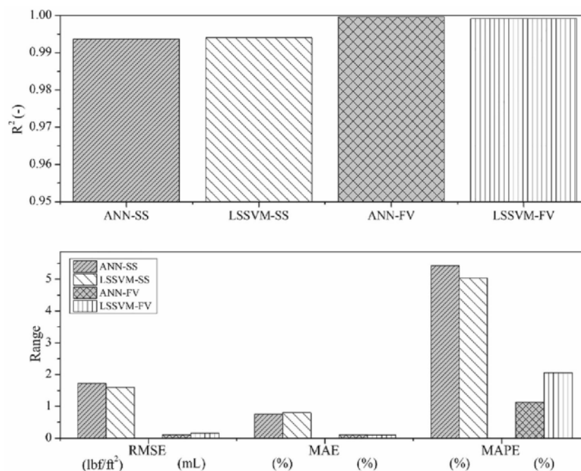
Fig. 21 Comparison of statistical parameters
