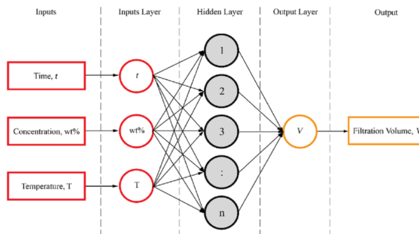
Fig. 5 ANN architecture for prediction of filtration volume
