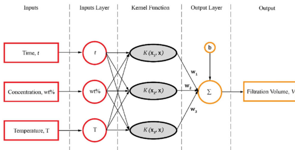
Fig. 7 LSSVM architecture for prediction of filtration volume
