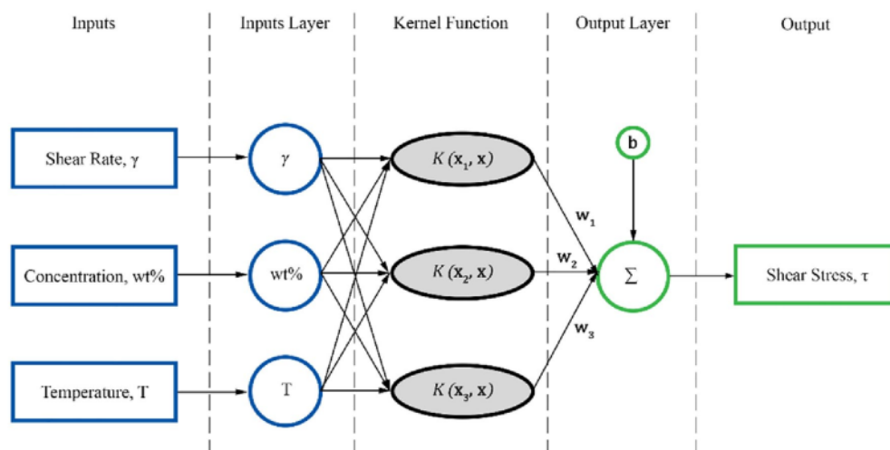
Fig. 6 LSSVM architecture for prediction of shear stress
