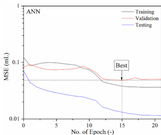
Fig. 15 MSE at different epochs of ANN for prediction of filtration volume
