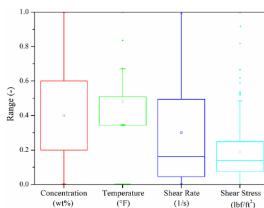
Fig. 2 Distribution of normalised data for prediction of shear stress
