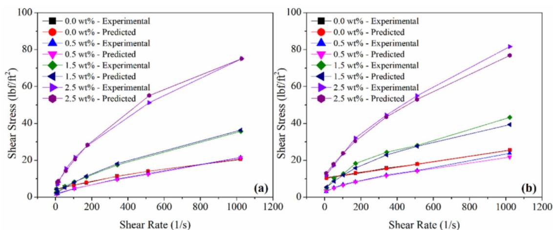
Fig. 22 Predicted and experimental rheo-gram. a 78 °F b 140 °F
