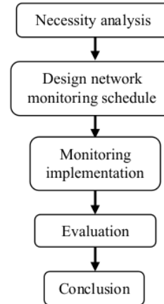
Fig 1. Research Method
