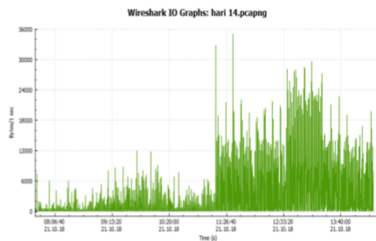
Fig. 6. The result graph of monitoring last day
