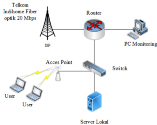
Fig. 3. Monitoring system scheme
