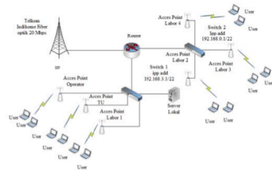
Fig. 2. Network topology in Telkom vocational school
