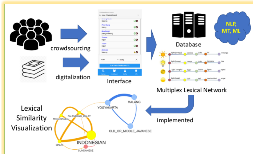
Figure 1: Proposed framework.
