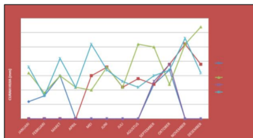
Fig 16. 2018 Rainfall Graph
