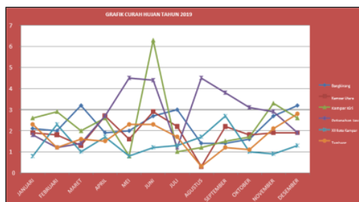
Fig 15. 2019 Rainfall Graph
