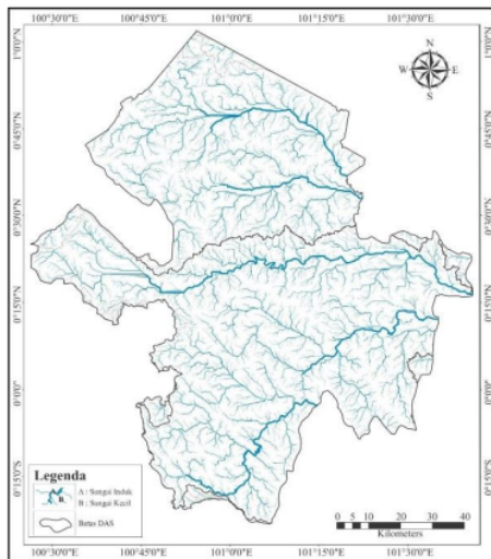
Fig 12. Watersheds map
