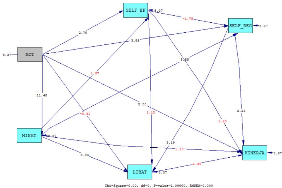
Figure 1. Path analysis with standardized
