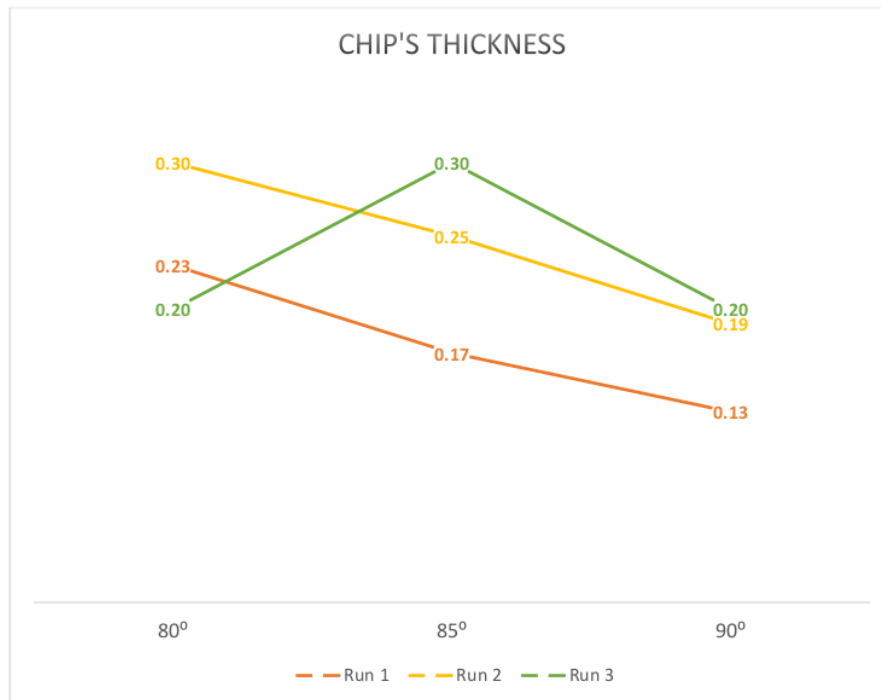
Figure 5. Chip thickness of varied tool's angle.
