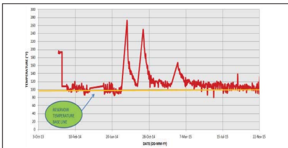
Figure 3 Graph YA23 well reservoir temperature data at long cyclic job (December 14 th , 2013 – November 22 th , 2015).
