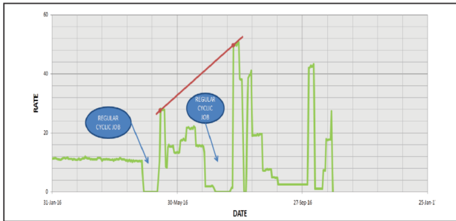
Figure 8 Graph of YA03 well oil production data on RUA field.
