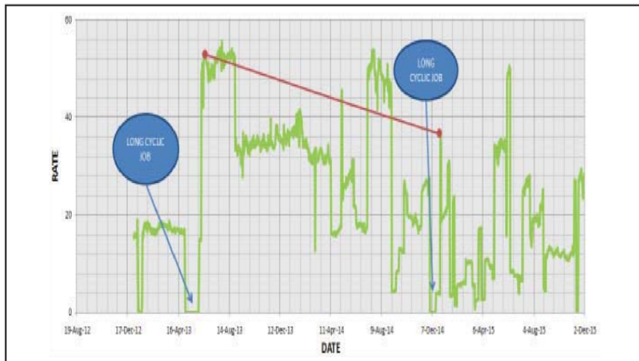
Figure 9 Graph of YA02 well oil production data on RUA field.
