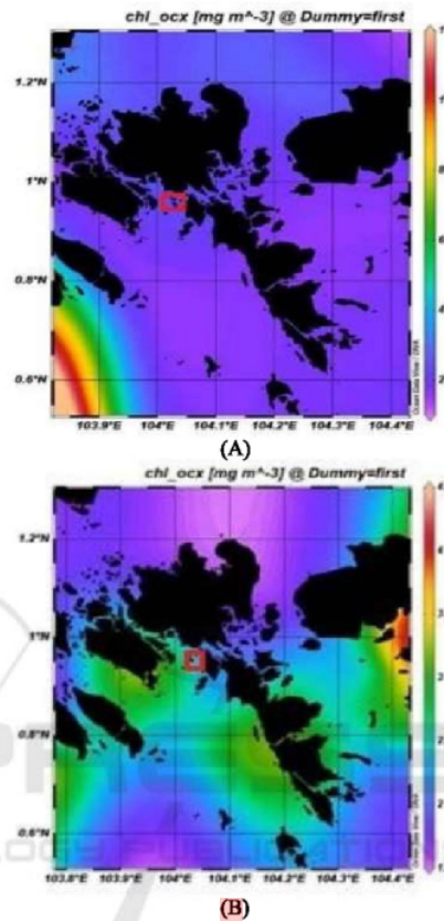
Figure 3: A. Chlorophyll A distribution (April 2020), B. Chlorophyll A distribution (May 2020).
