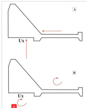
Figure 18: Uplift-pressure of MT
