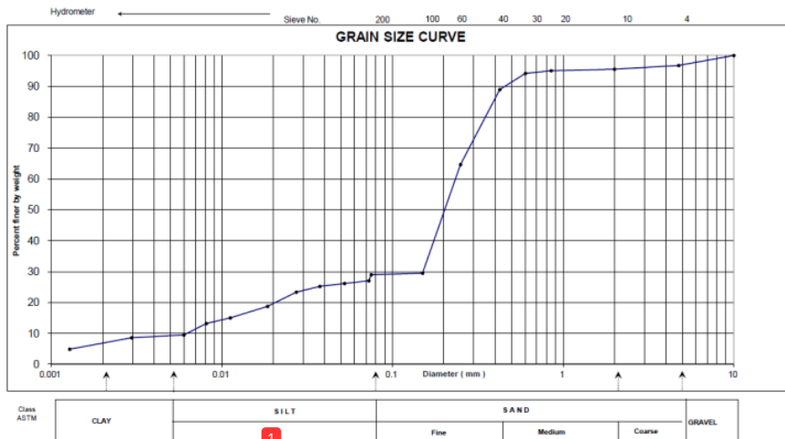
Figure 6: The grain size curve of HB.2
