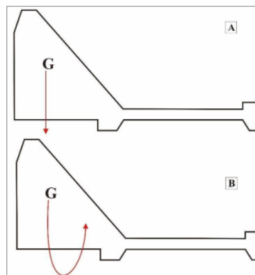
Figure 12: Own gravity on the weir
