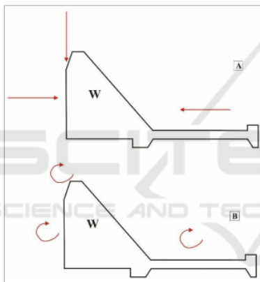
Figure 15: A hydrostatic force of MG
