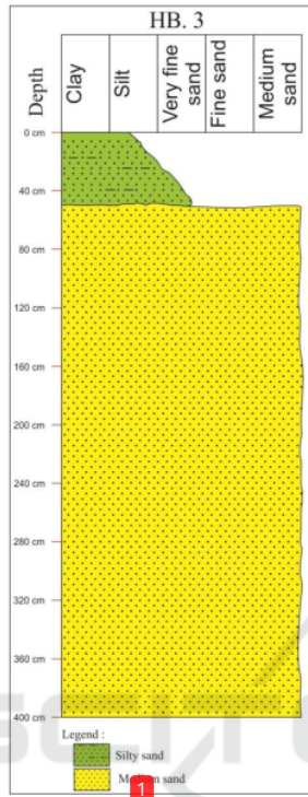
Figure 5: The sediment log at HB.3
