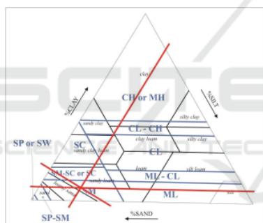
Figure 7: Type soil in HB.2
