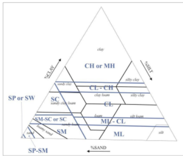
Figure 3: The USCS triangle
