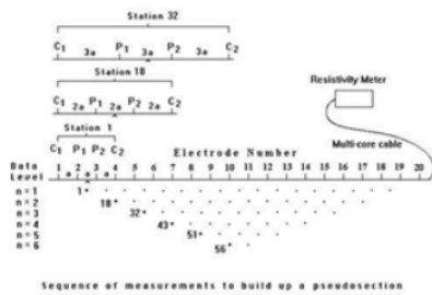
Figure 4: Equipment set up to acquisition resistivity data(Loke and Barker, 1995)
