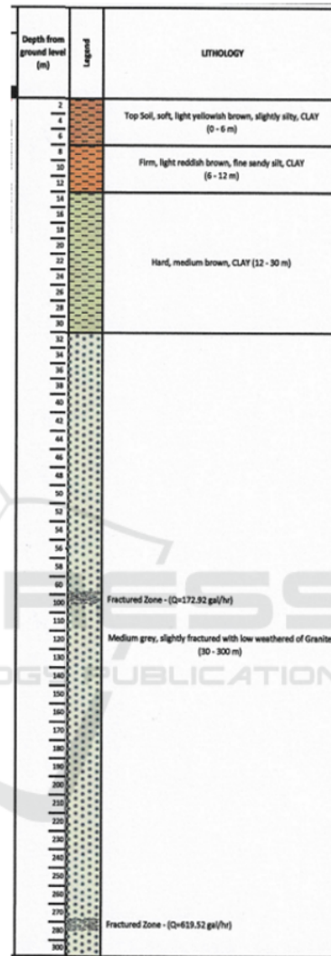
Figure 8: Drilling data of PDL 6
