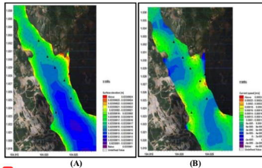
1 Fig. 8. Modeling of the final (A) water surface elevation, (B) current flow during water filling process before the water discharge from the outlet.
