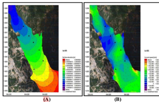
1 Fig. 7. Modeling of the beginning (A) water surface elevation, (B) current flow during water filling process before the water discharge from the outlet.
