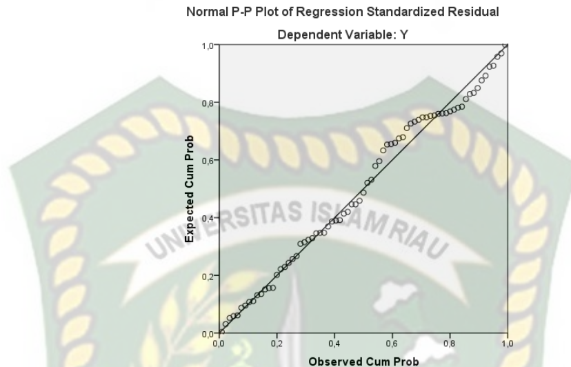
Gambar 5.2 Normal Probability Plot
