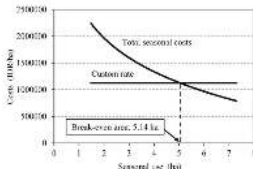
Fig. 5 Break-even analysis for rotary tillers
