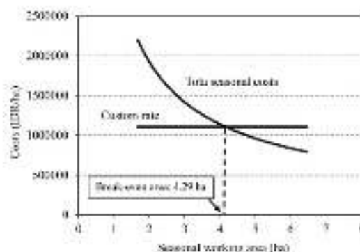
Fig. 6 Break-even analysis for moldboard plows
