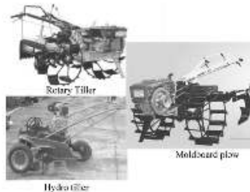
Fig. 1. Three types of power tillers
