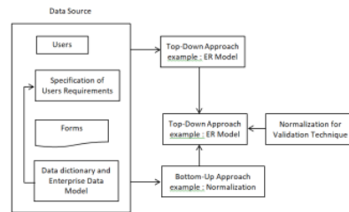
Figure 1: Role of normalization in database design.
